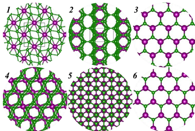
Figure 28. Crystal structures of the Mn–B phases found using the evolutionary calculations: (1) Pnnm -MnB 4 , (2) Pm -MnB 13 , (3) P\bar{6}m2 -MnB 3 , (4) P2_1/c -MnB 4 , (5) R\bar{3}m -MnB 4 , (6) P\bar{6}m2 -MnB 5 .
