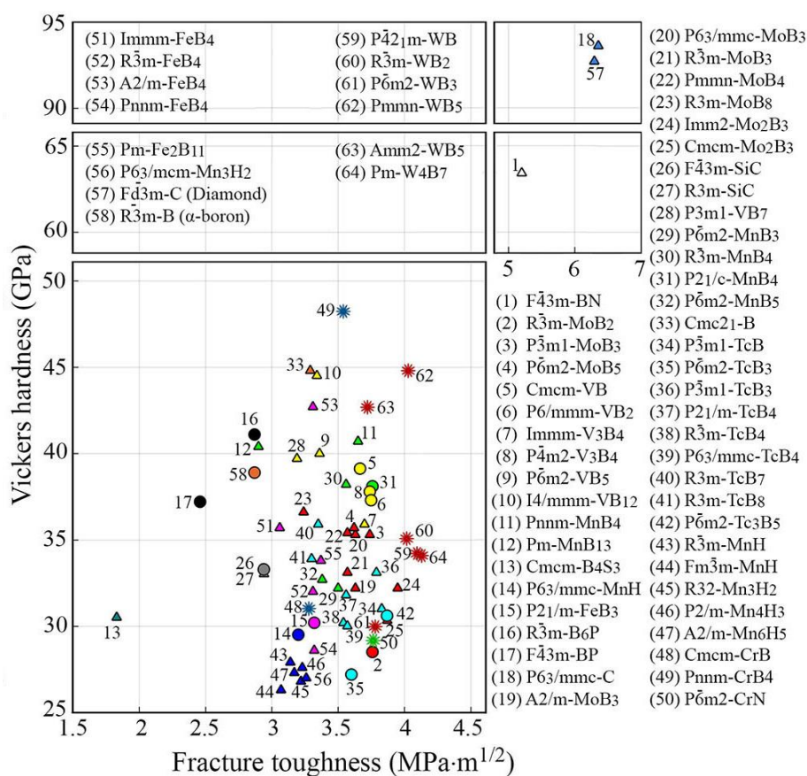
Figure 34. 2D plot of the Vickers hardness vs. fracture toughness. Stable hard compounds from the previous works 24, 25 are shown as “suns”; stable and metastable compounds found in this work are represented by circles and triangles, respectively.
