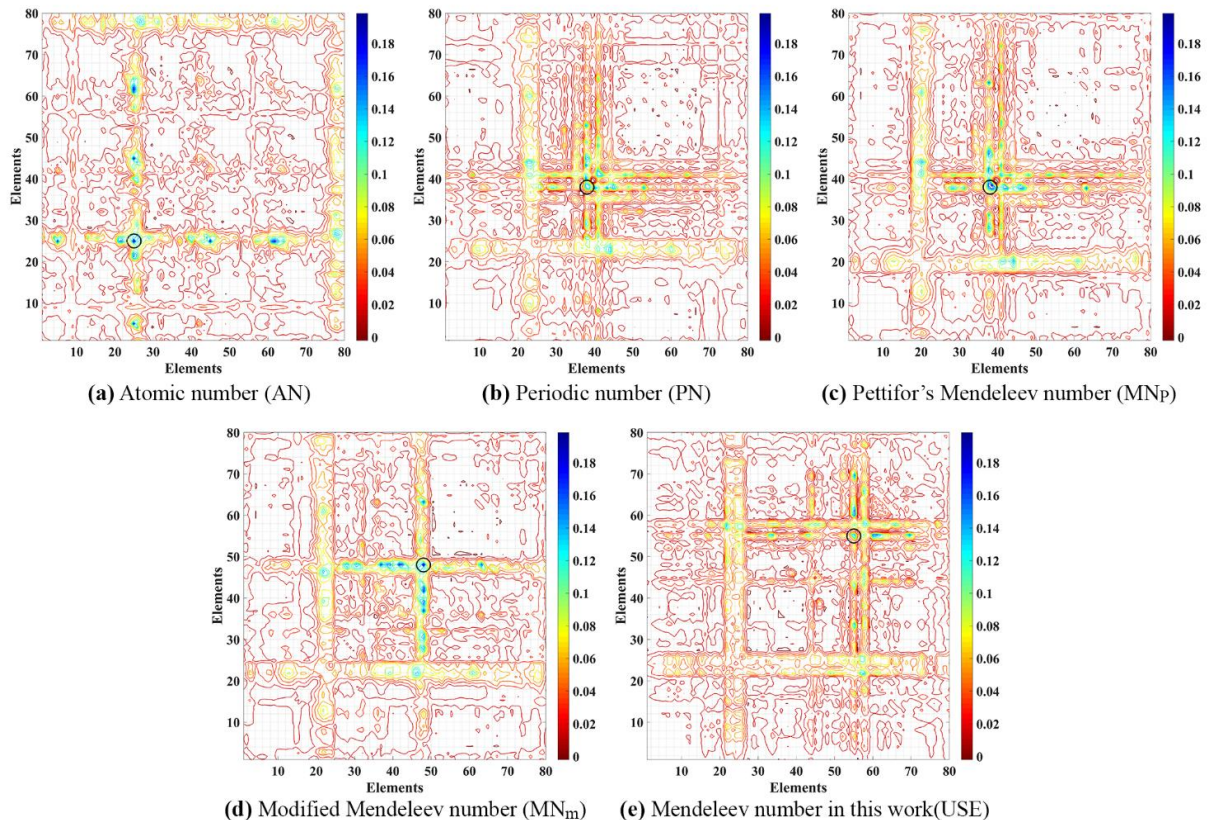
Figure 17. 2D maps of magnetization (in the unit of \mu_B \text{Å}^{-3} ) of binary systems, plotted in various MNs. The representative for each binary system is the phase with the highest magnetization in our database. The material with the highest magnetization is shown by black hollow circle.
